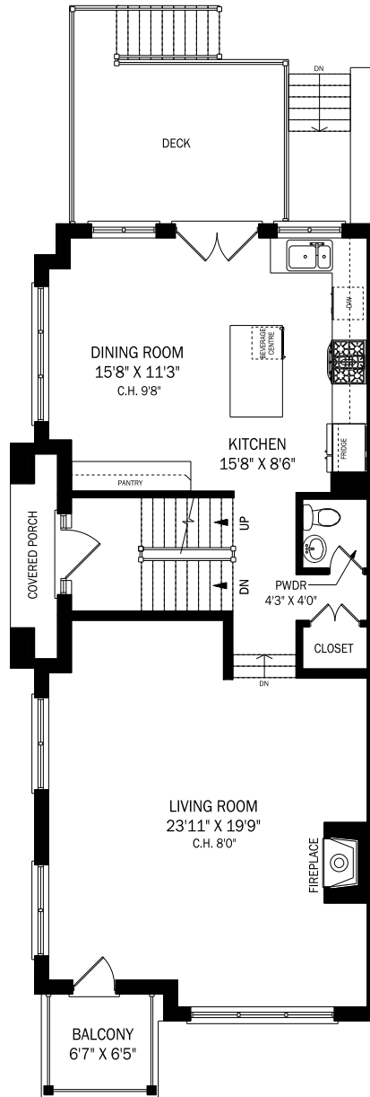
MAIN LEVEL - 1034 SQUARE FEET
